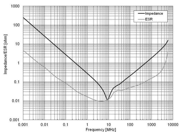
④3225X7RB226MS
