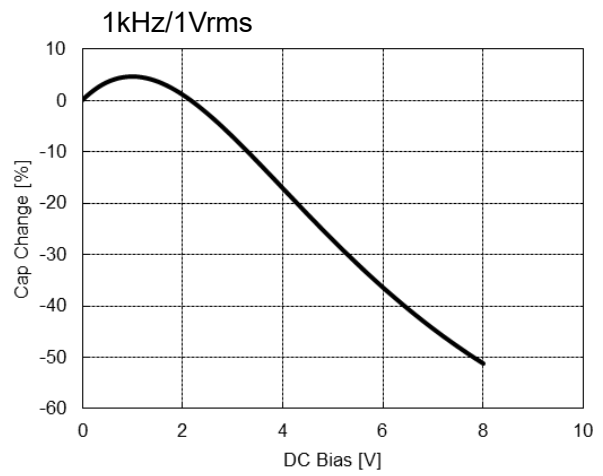
④3225X7RB226MS
