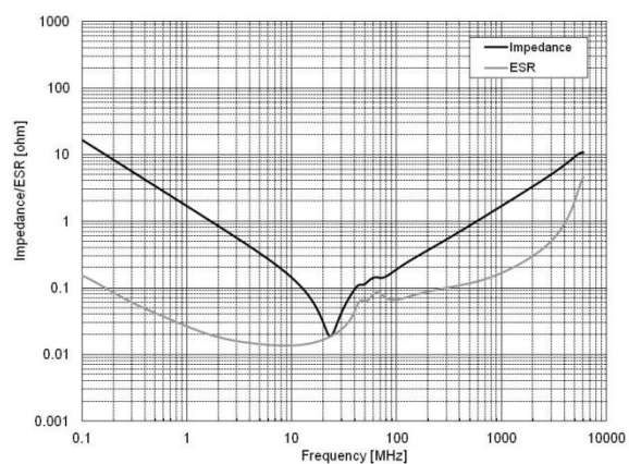
③3216X7RA226MS
