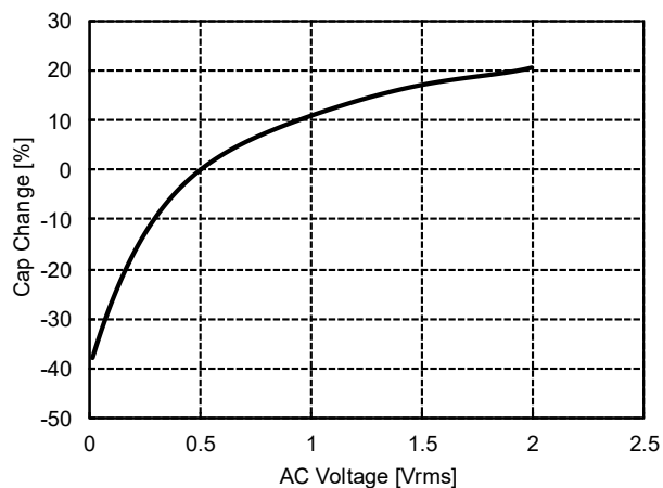
⑤1005X7SB104KR
