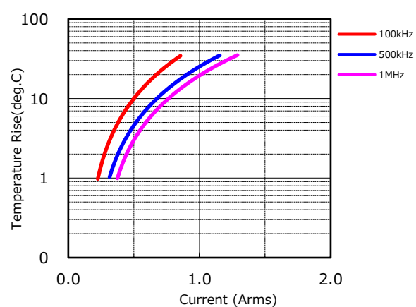
⑤1005X7SB104KR
