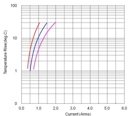
③3216X7RA226MS
