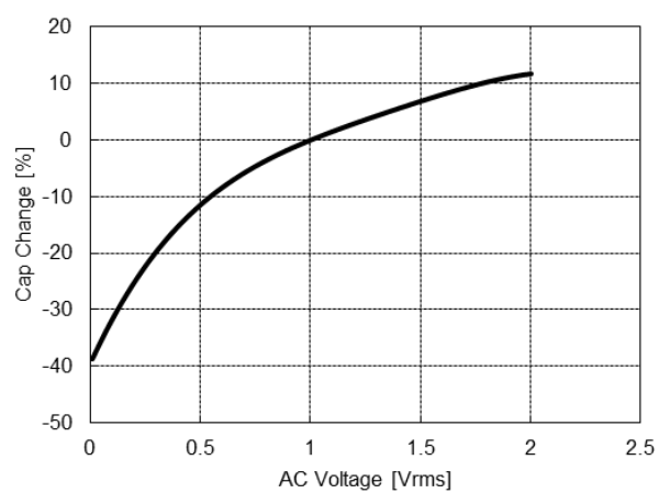
④3225X7RB226MS
