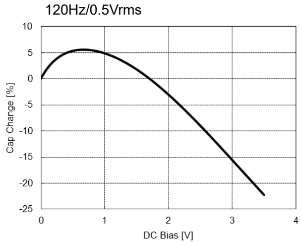
⑤1005X7SB104KR
