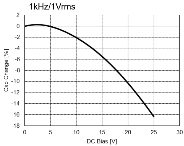
③3216X7RA226MS
