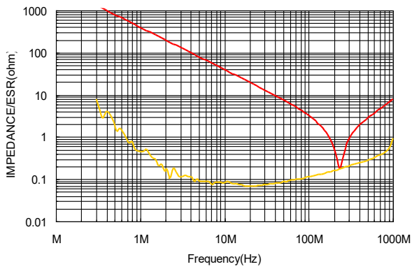
③N2040/L104-3216C0G2D391J
