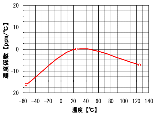
③ N2040/L104-3216C0G2D391J
