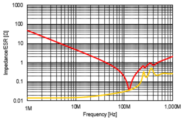
A. N2040/L104N1608C0G1H332J
