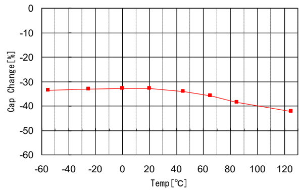
B. N2040/L104N2012C0G2A182J
