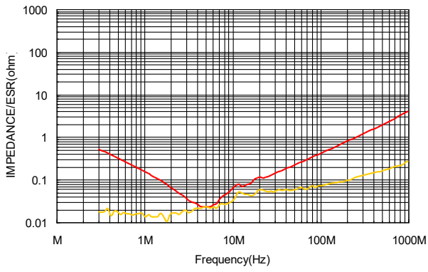
⑦N2040/L104-5750X7R1H105K
