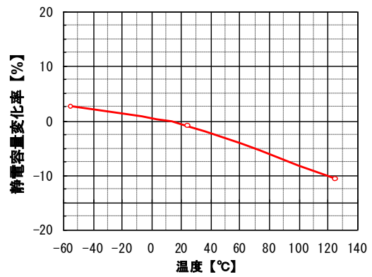
④ N2040/L104-3225X7R1E105K
