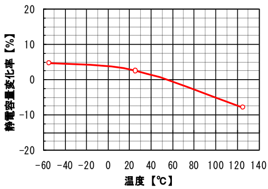
⑨ N2040/L104-5750X7R2A474K
