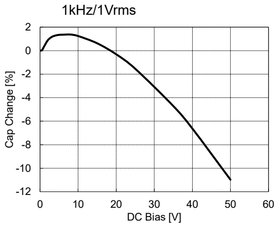
⑥ N2040/L104-5750X7R1H474K
