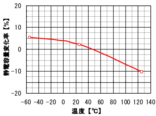
⑦ N2040/L104-5750X7R1H105K
