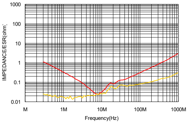
⑨N2040/L104-5750X7R2A474K
