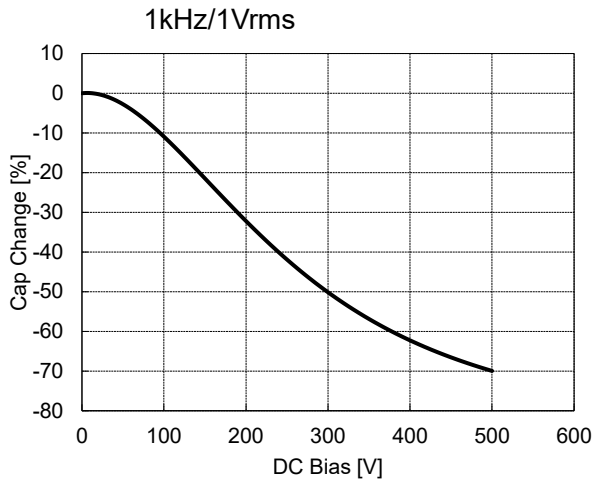
⑪ N2040/L104-5750X7R2H104K
