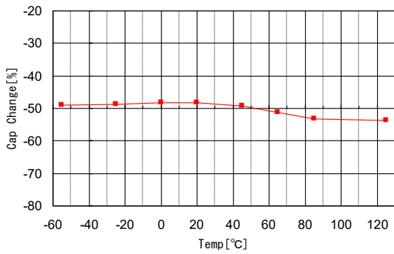
A.N2040/L104N1608C0G1H332J
