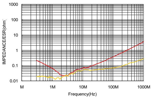
⑤N2040/L104-4532X7R1E225K
