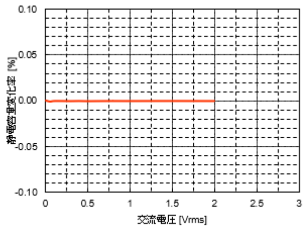
A.N2040/L104N1608C0G1H332J
