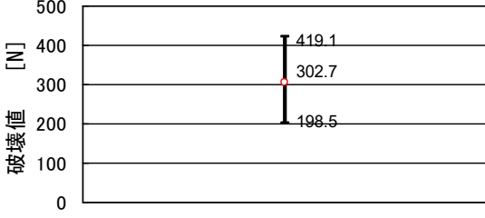
⑧N2040/L104-5750X7R2A224K
