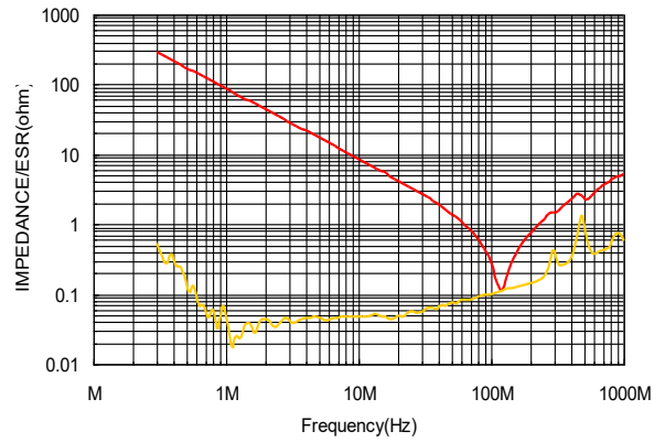
②N2040/L104-3216C0G2A182J
