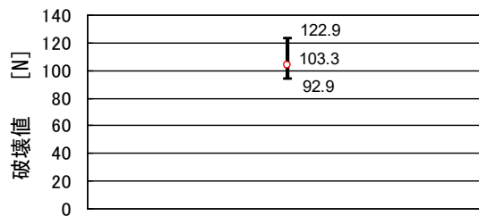
③N2040/L104-3216C0G2D391J
