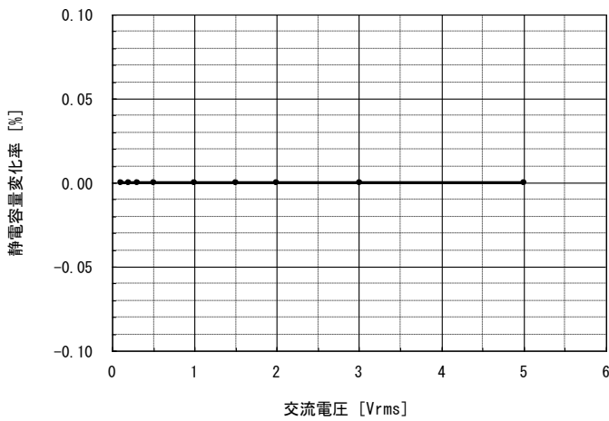
③N2040/L104-3216C0G2D391J
