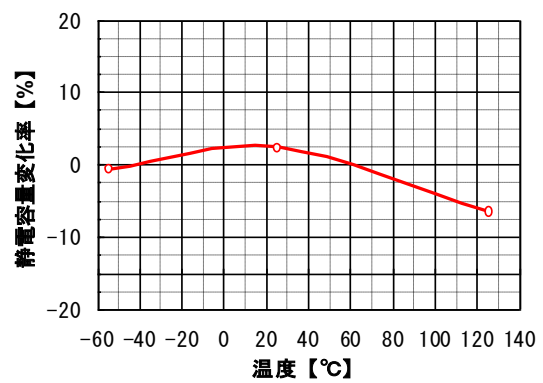
⑥ N2040/L104-5750X7R1H474K
