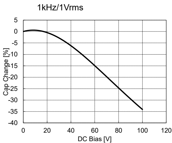
⑨ N2040/L104-5750X7R2A474K
