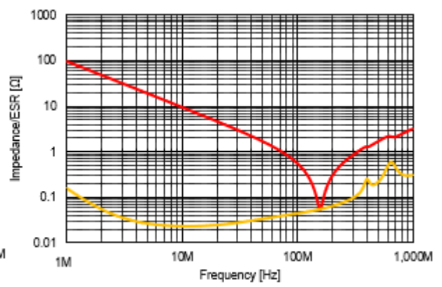
B. N2040/L104N2012C0G2A182J
