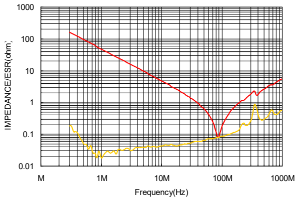
①N2040/L104-3216C0G1H332J
