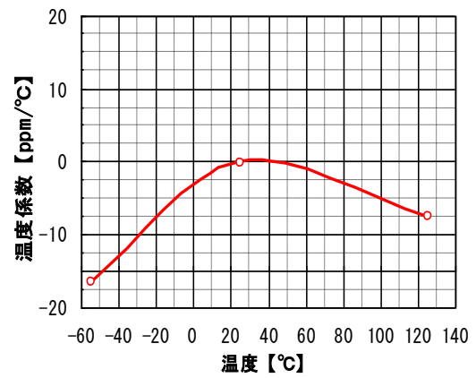
② N2040/L104-3216C0G2A182J
