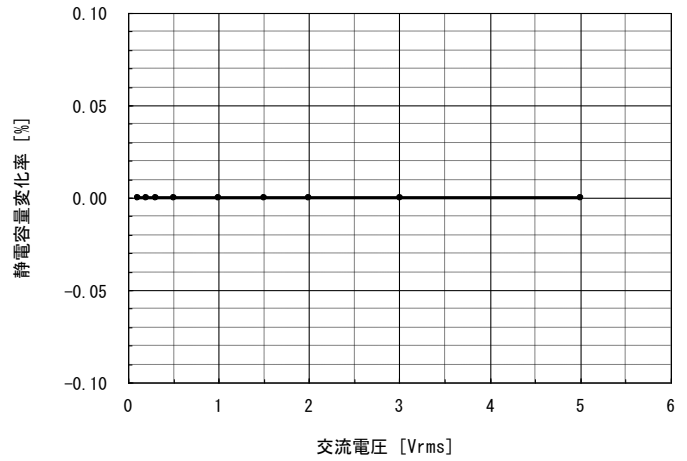
②N2040/L104-3216C0G2A182J
