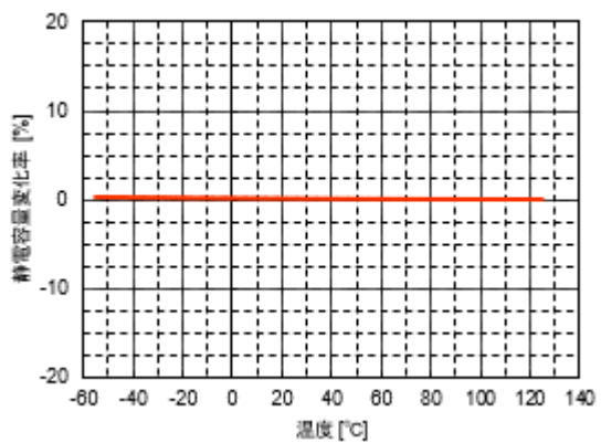
A. N2040/L104N1608C0G1H332J
