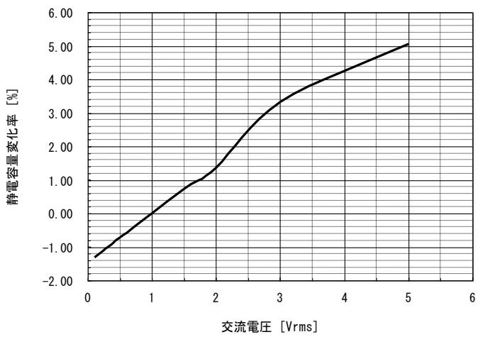
⑧N2040/L104-5750X7R2A224K
