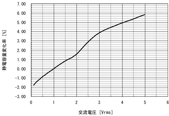
⑦N2040/L104-5750X7R1H105K
