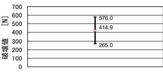
⑨N2040/L104-5750X7R2A474K
