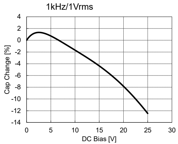
⑤ N2040/L104-4532X7R1E225K
