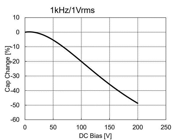
⑩ N2040/L104-5750X7R2D224K
