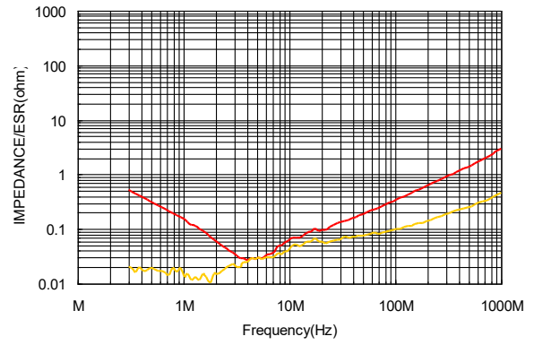
④N2040/L104-3225X7R1E105K
