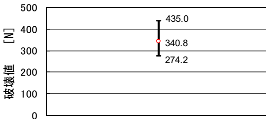
⑥N2040/L104-5750X7R1H474K
