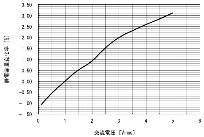
⑩N2040/L104-5750X7R2D224K
