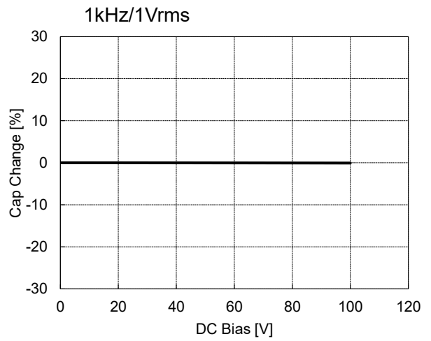
B.N2040/L104N2012C0G2A182J
