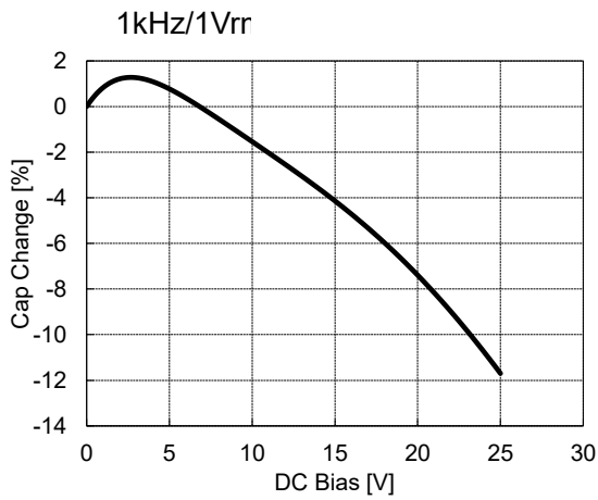
④ N2040/L104-3225X7R1E105K
