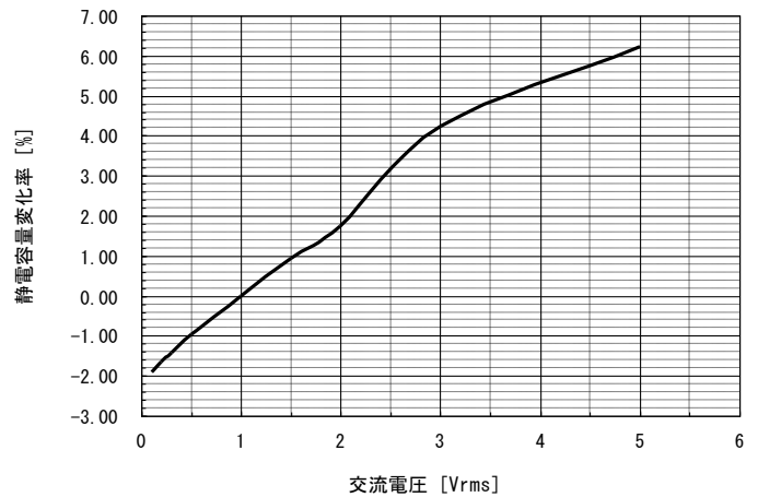
⑥N2040/L104-5750X7R1H474K
