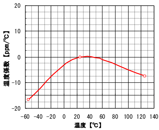
① N2040/L104-3216C0G1H332J
