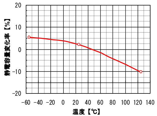
⑧ N2040/L104-5750X7R2A224K
