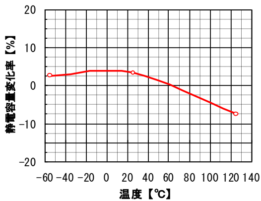
⑪ N2040/L104-5750X7R2H104K
