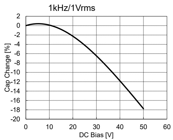
⑦ N2040/L104-5750X7R1H105K
