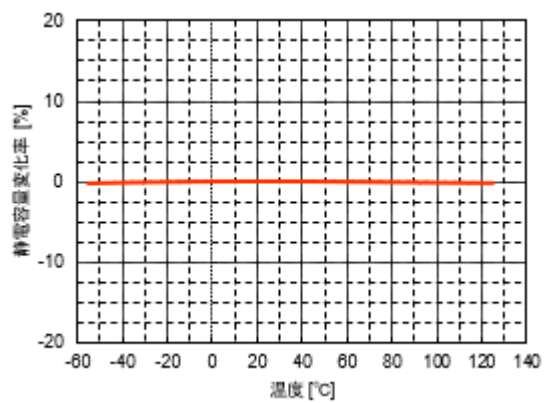
B. N2040/L104N2012C0G2A182J
