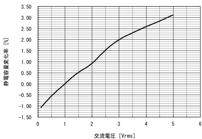
⑩N2040/L104-5750X7R2D224K
