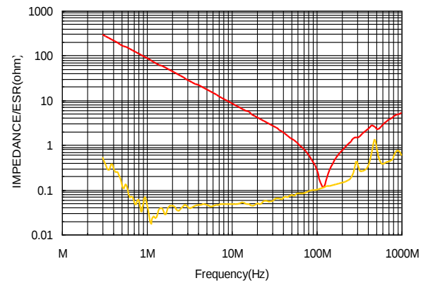
②N2040/L104-3216C0G2A182J
