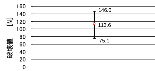
④N2040/L104-3225X7R1E105K
