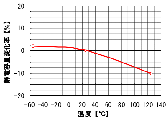
⑤ N2040/L104-4532X7R1E225K
