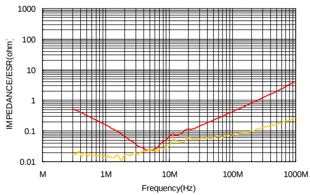
⑦N2040/L104-5750X7R1H105K
