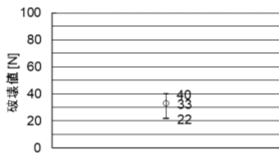
A. N2040/L104N1608C0G1H332J
