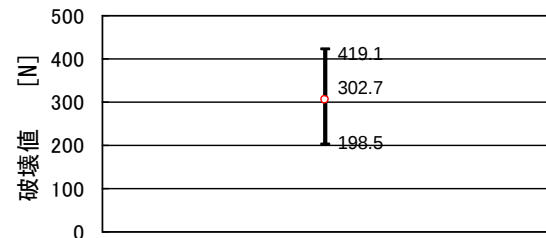
⑧N2040/L104-5750X7R2A224K
