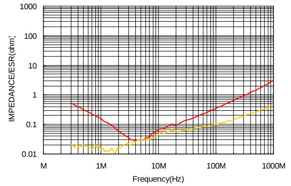
④N2040/L104-3225X7R1E105K
