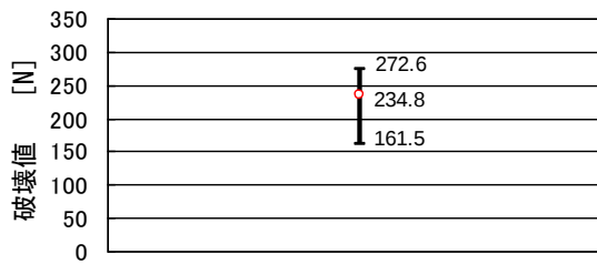
⑤N2040/L104-4532X7R1E225K
