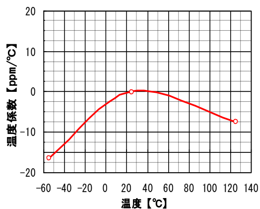
② N2040/L104-3216C0G2A182J
