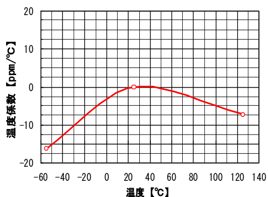
③ N2040/L104-3216C0G2D391J
