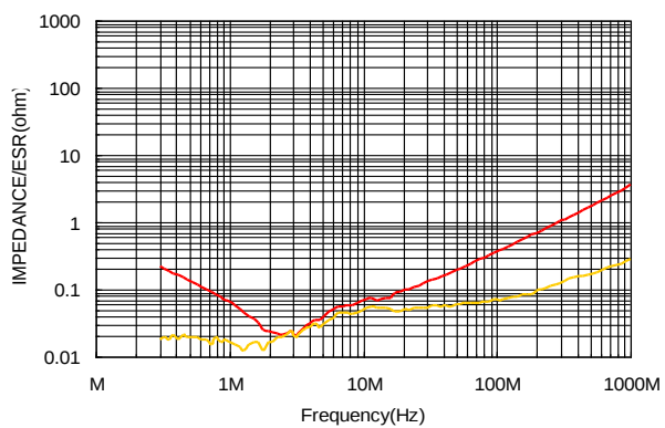
⑤N2040/L104-4532X7R1E225K
