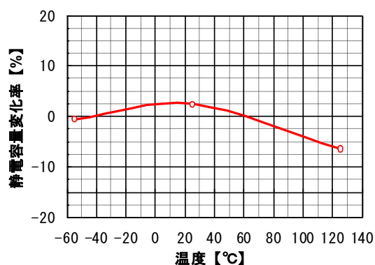
⑥ N2040/L104-5750X7R1H474K
