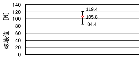
①N2040/L104-3216C0G1H332J
