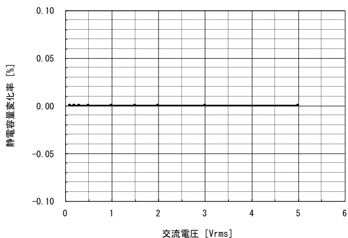
③N2040/L104-3216C0G2D391J
