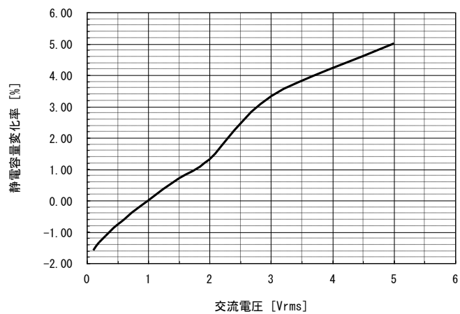
⑨N2040/L104-5750X7R2A474K
