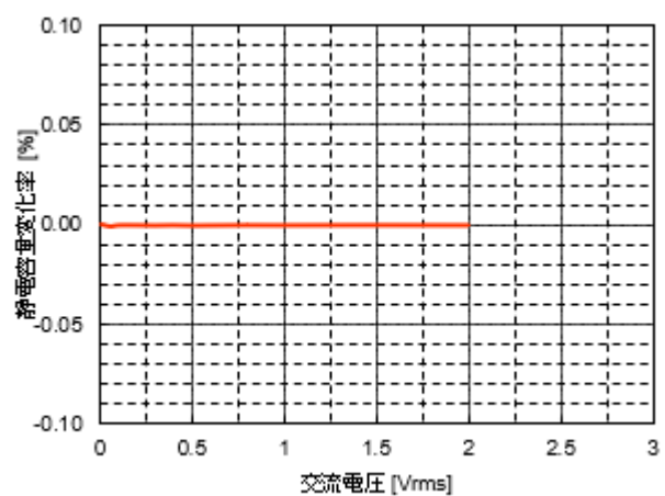
A.N2040/L104N1608C0G1H332J
