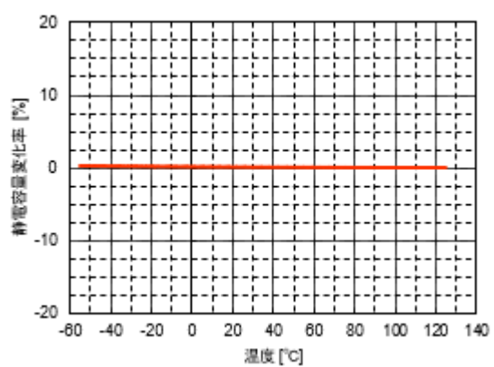
A. N2040/L104N1608C0G1H332J
