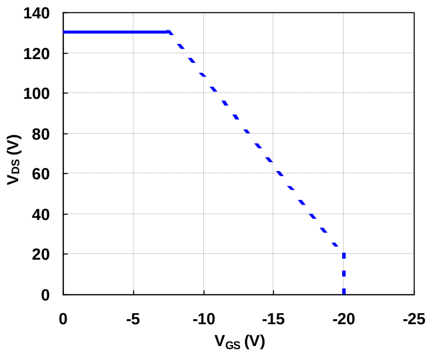
図 45 SEE-SOA (JAXA R 2SK4152, 2SK4153, 2SK4154)
