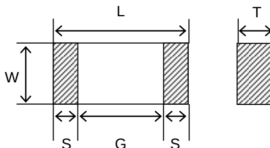
Figure L-1. Externals
